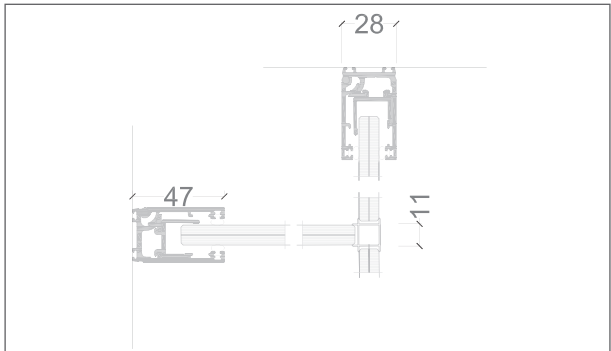
"T" JUNCTION
